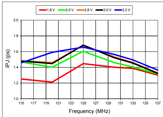
Figure 13. RMS Integrated Phase Jitter Random (12k to 20 MHz) vs Frequency [9]
